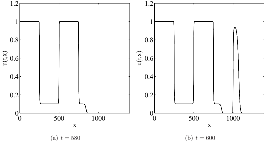
Figure 1: Profile of the solution u(t, x) , at two successive times, t = 580 and t = 600 , starting from a compactly supported initial condition u(0, x) and with \mu^+ = 1 , \mu^- = 0.1 , D = 1 , \theta = 1/2 and L = 500 .
